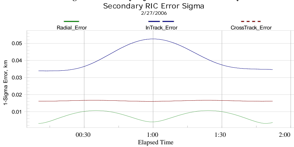
Figure 12. Secondary object Covariance time history.
